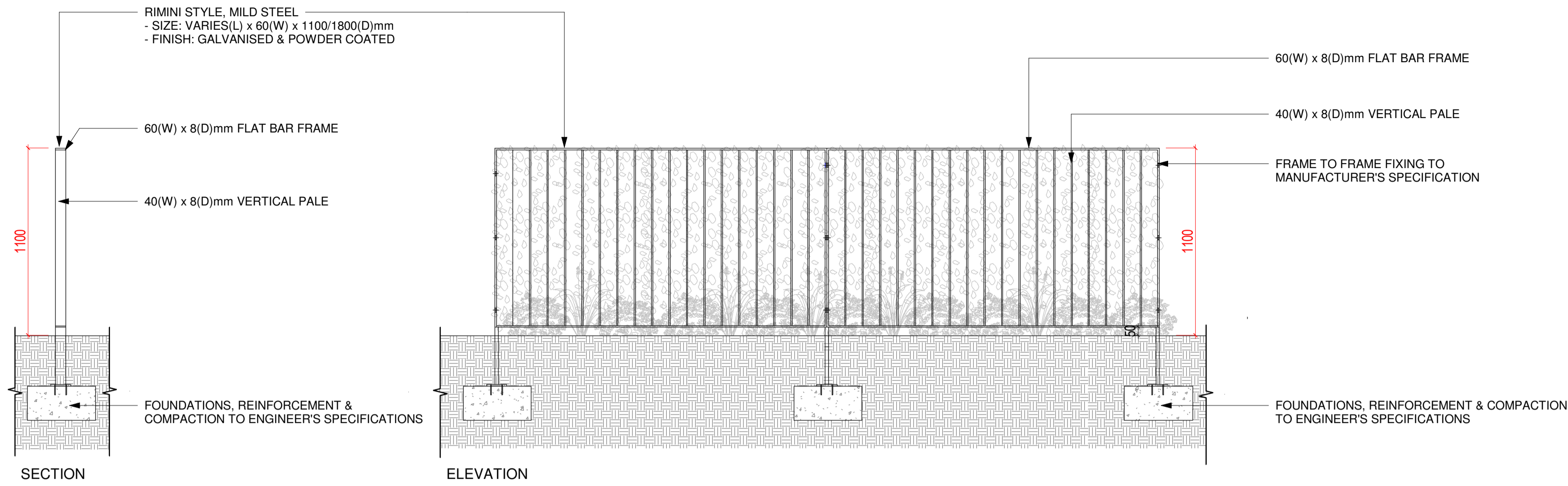
1 TYPICAL DETAIL: 1.1m HIGH METAL RAILING SCALE: 1 : 20 @A1
