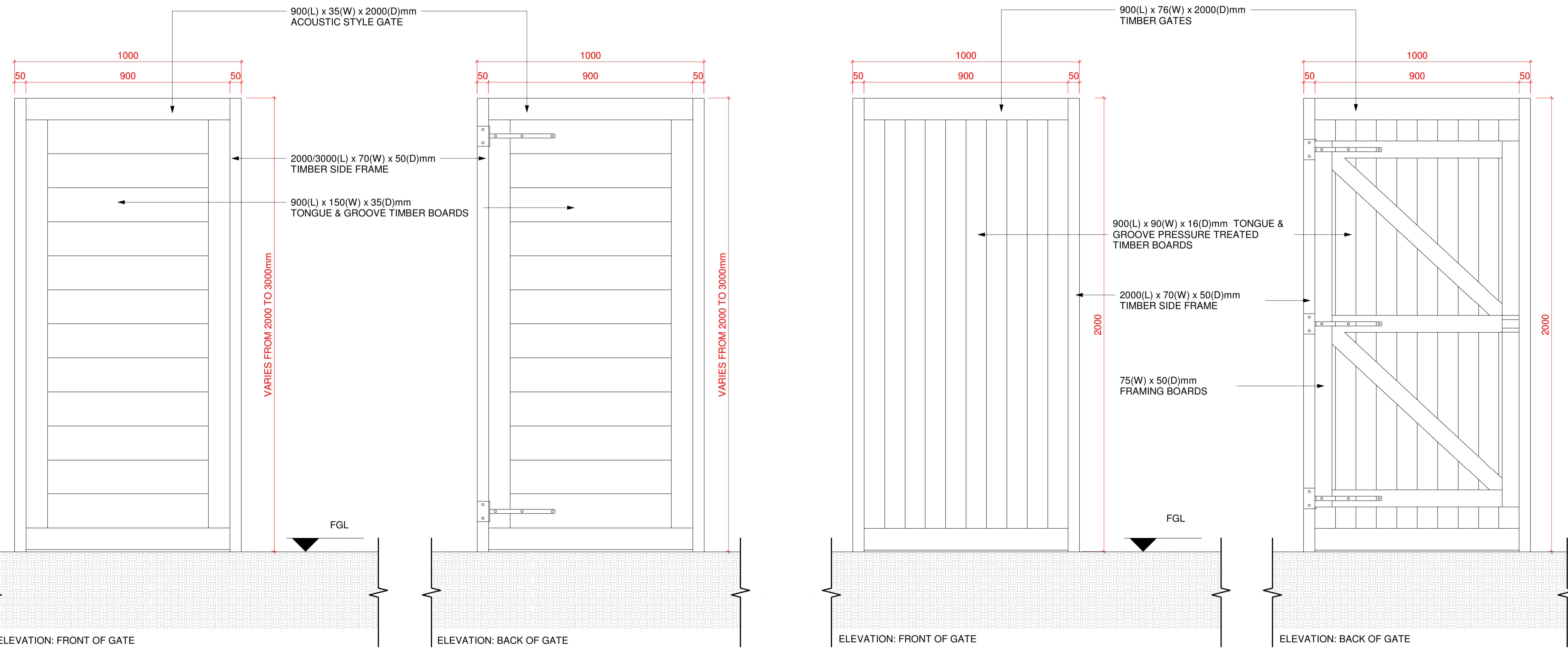
2 TYPICAL DETAIL: ACOUSTIC FENCING STYLE GATES SCALE: 1 : 10 @A1
